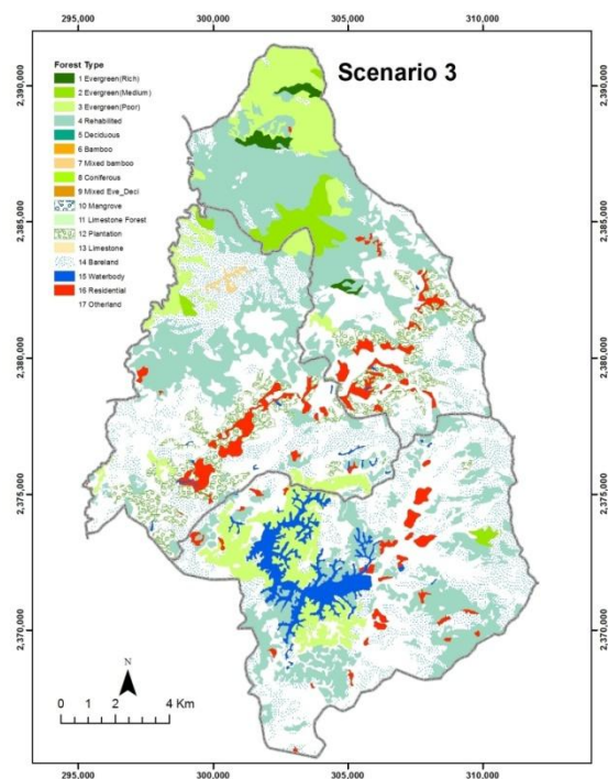
Figure 3. Scenario 3
